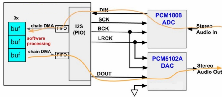
Figura 11: Datapath audio
